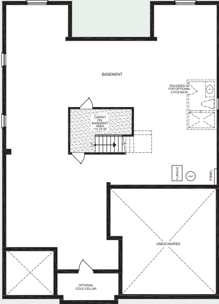
BASEMENT Elevation A, B & C
