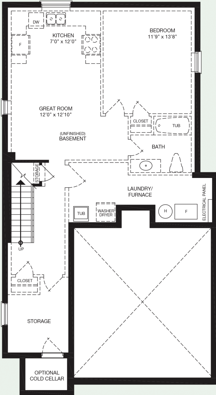
BASEMENT ROUGH-IN LAYOUT Elevation A, B, C
