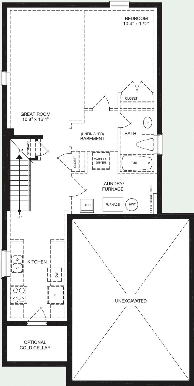
BASEMENT ROUGH-IN LAYOUT Elevation A, B, C
